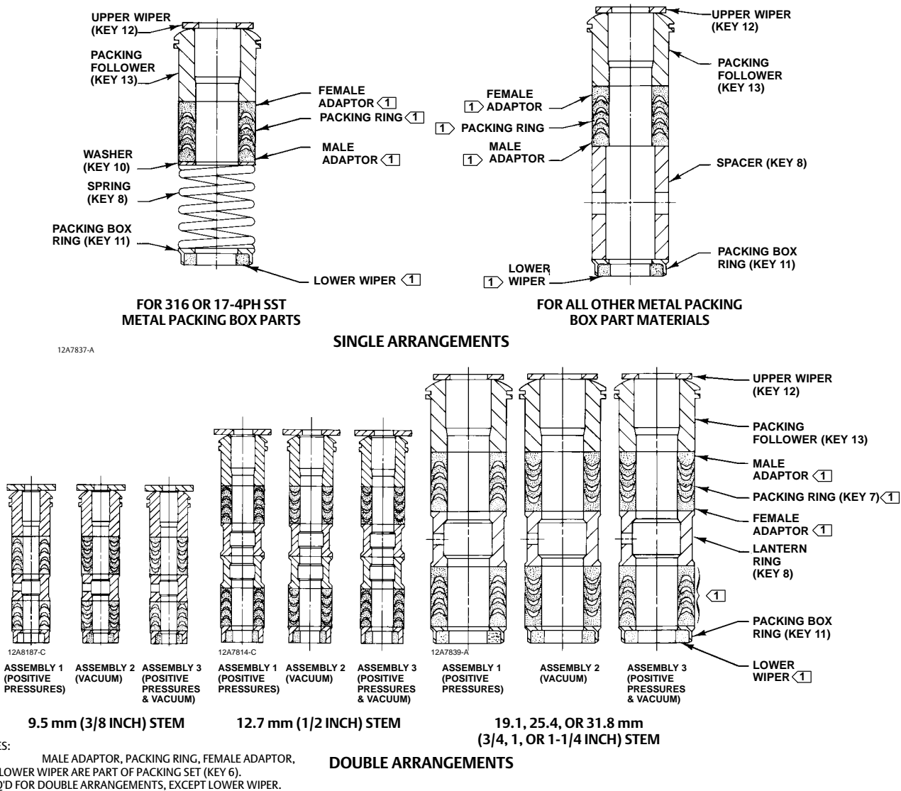
Figure 3. PTFE V-Ring Packing Arrangements for Plain or Extension Bonnets
