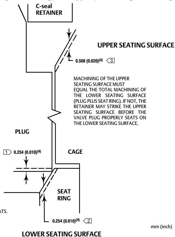
Figure 11. Example of Machining the Lower (Valve Plug to Seat Ring) and Upper (C-seal Plug Seal to Cage) Seating Surfaces
