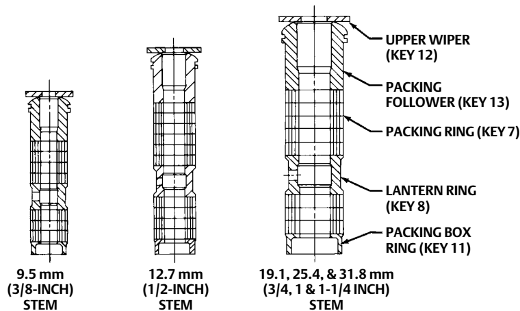
Figure 4. PTFE/Composition Packing Arrangements for Plain or Extension Bonnets
