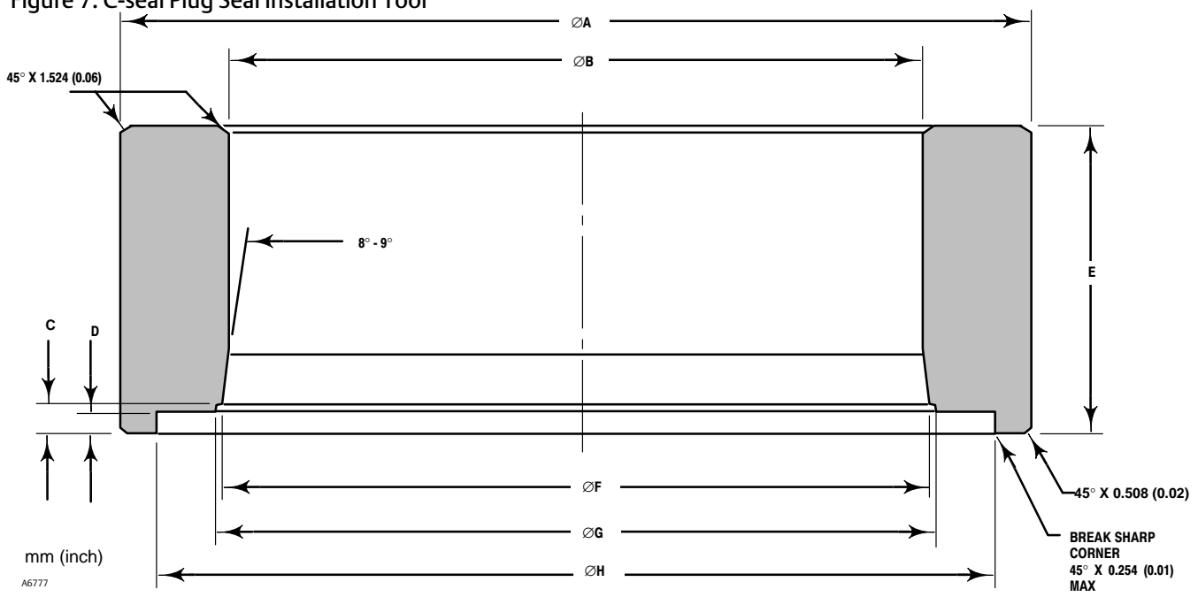
Figure 7. C-seal Plug Seal Installation Tool
