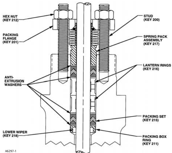
Figure 15. Typical ENVIRO-SEAL Packing System with PTFE Packing
