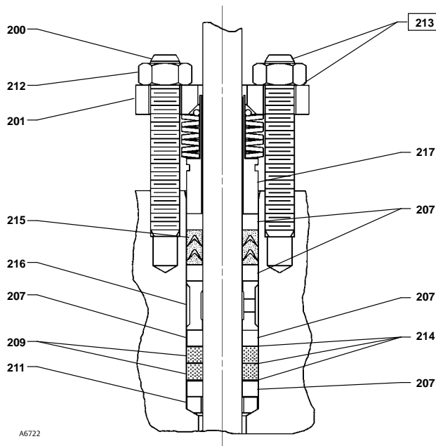
Figure 17. Typical ENVIRO-SEAL Packing System with Duplex Packing
